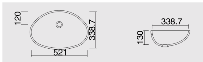
FONTANA FD-510 521 x 338.7 x 130 mm
