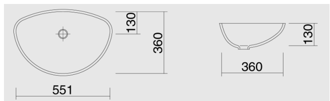
FONTANA FD-560 551 x 360 x 130 mm
